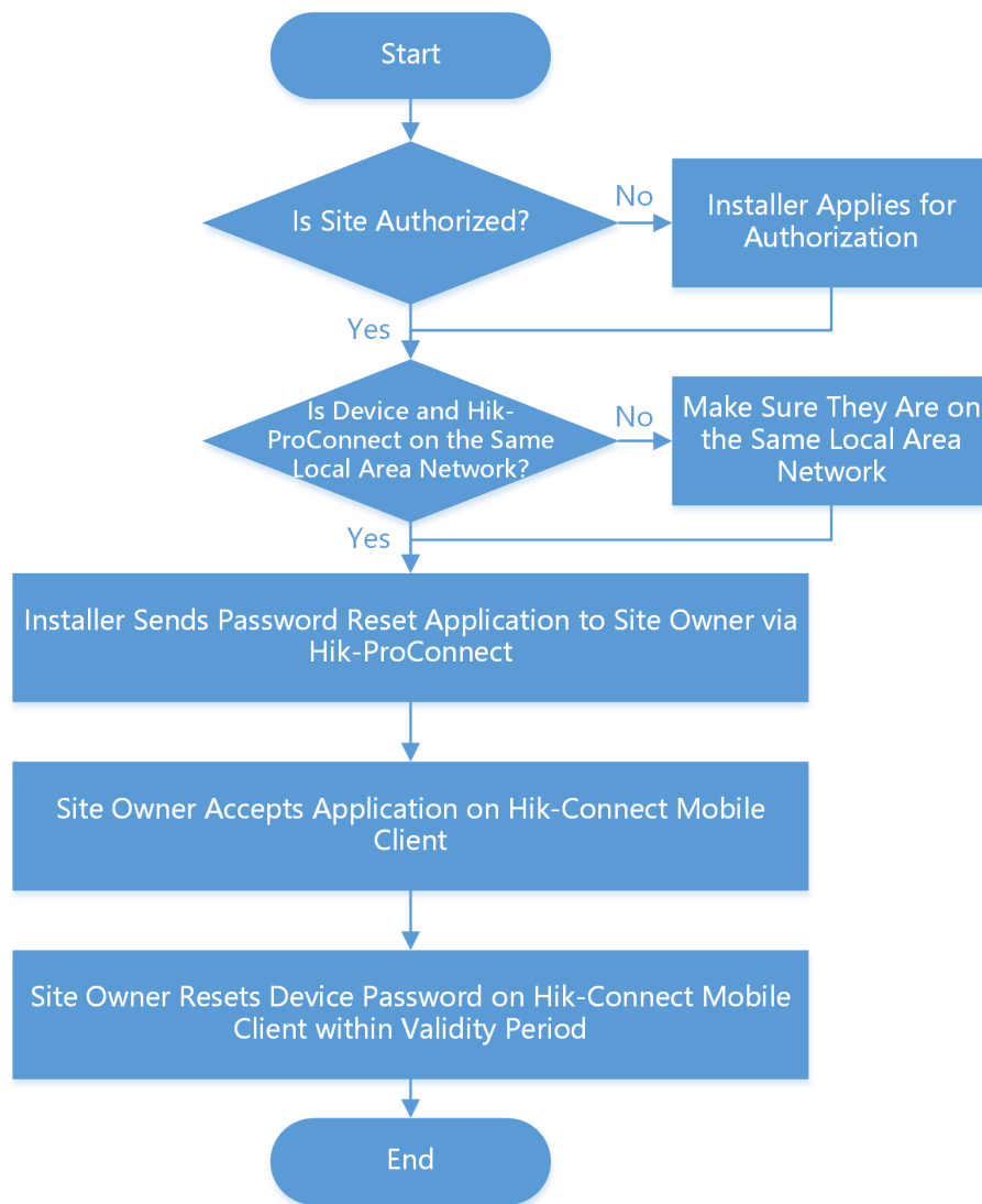
Figure 6-4 Flow Chart of Resetting Device Password
